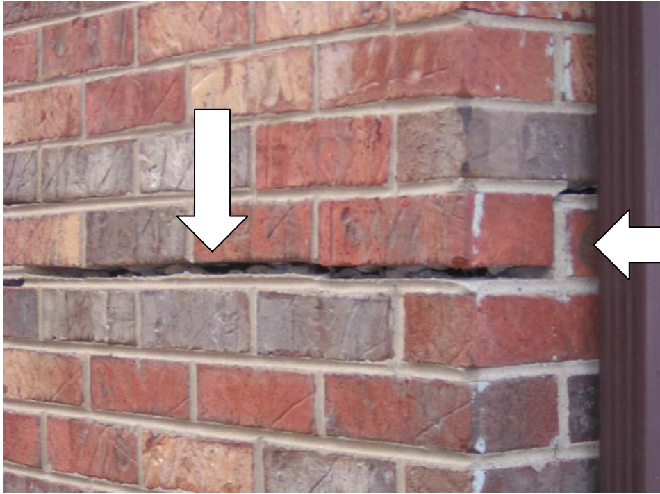
Crack in brick veneer before the foundation lifting process.
