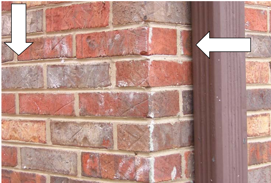
The crack in the brick veneer is now almost completely closed after the lifting process.
